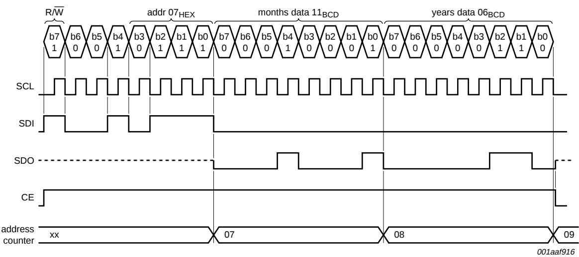
Fig 20. Serial bus read example
