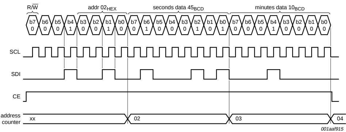
Fig 19. Serial bus write example
