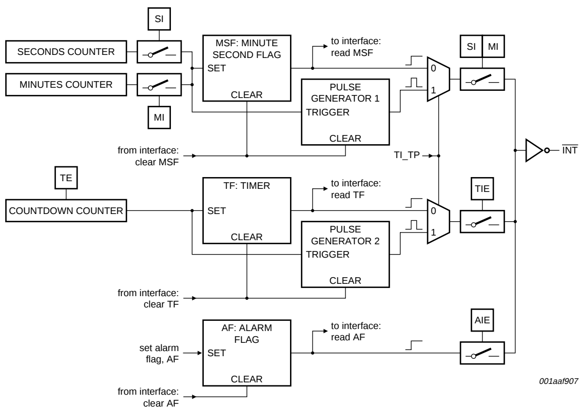
Fig 11. Interrupt scheme
